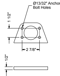
Surface Mount Base
