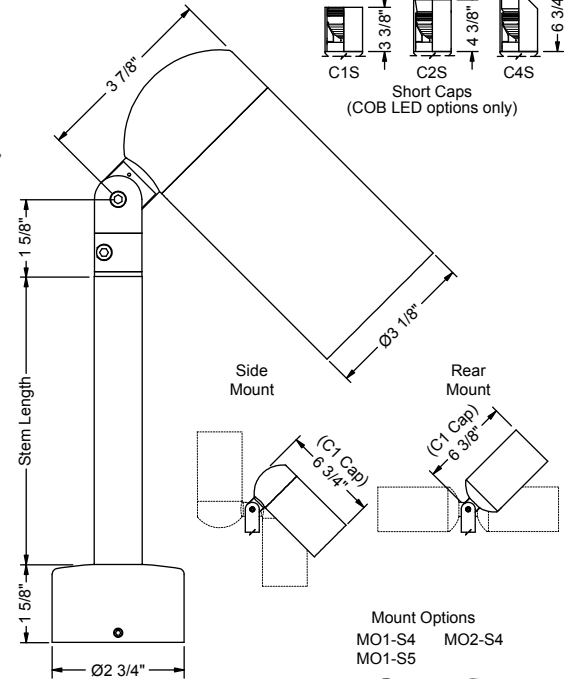
PA12 shown with: SM head, K2 knuckle, C1 cap, S1 style, & MO1 mount cap.
